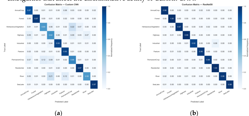
Figure 5. Normalized confusion matrices for (a) Custom CNN and (b) ResNet50 on EuroSAT.
