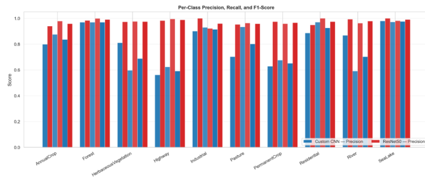
Figure 4. Per-class precision, recall, and F1-score: Custom CNN vs ResNet50.
