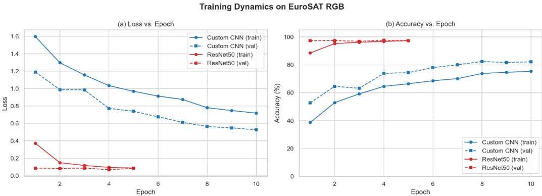
Figure 3. Training and validation curves for Custom CNN (10 epochs) and ResNet50 (5 epochs).
