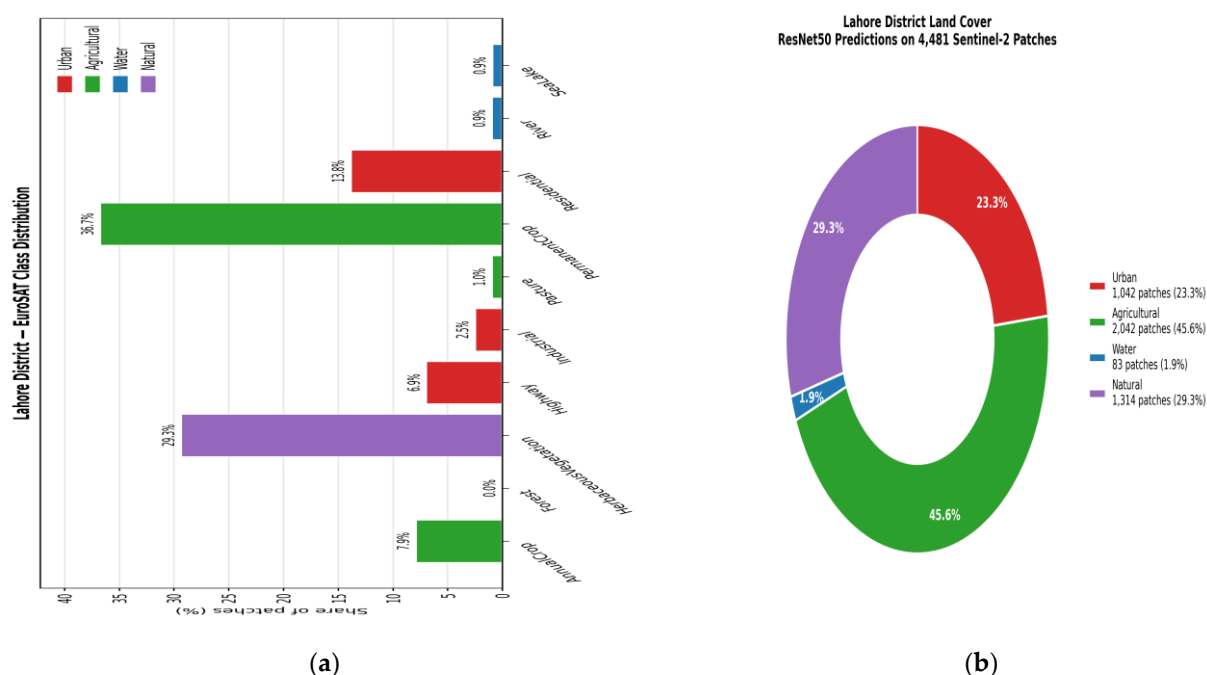
Figure 9. Land cover distribution in Lahore District predicted by ResNet50: (a) EuroSAT class-wise share; (b) aggregated 4-bin LULC composition.
